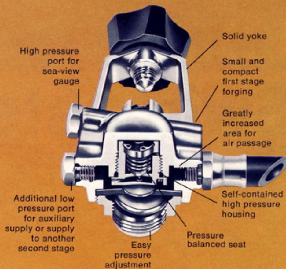
FIRST STAGE MR12
