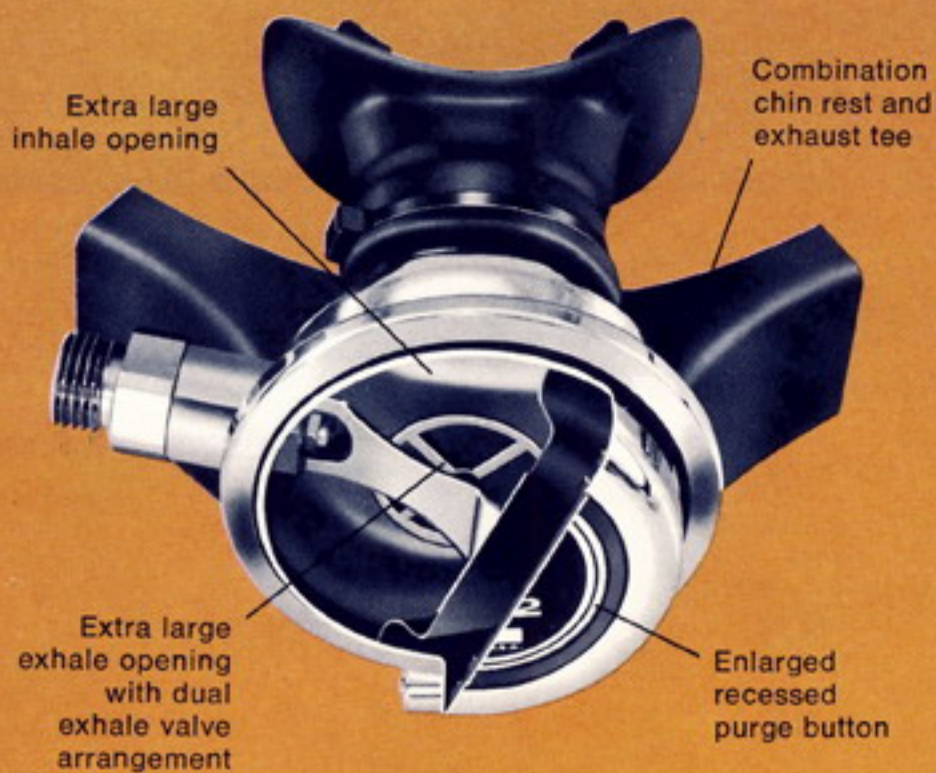
SECOND STAGE R12J & MR12
