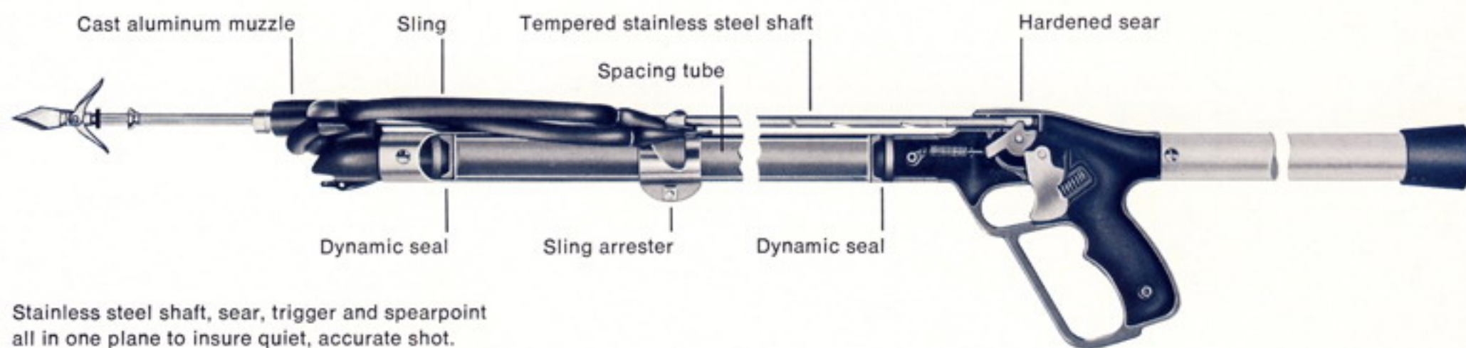
CUTAWAY ILLUSTRATION OF SWIMASTER GUN
